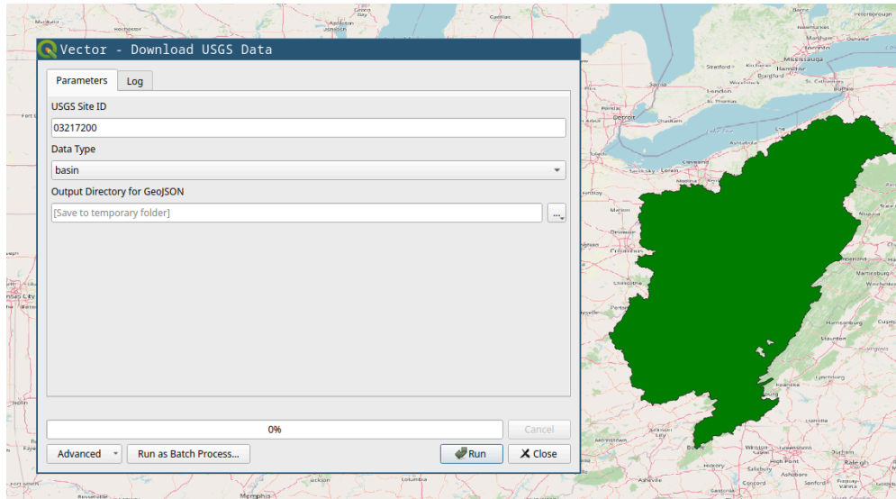
Figure 2: QGIS Download
